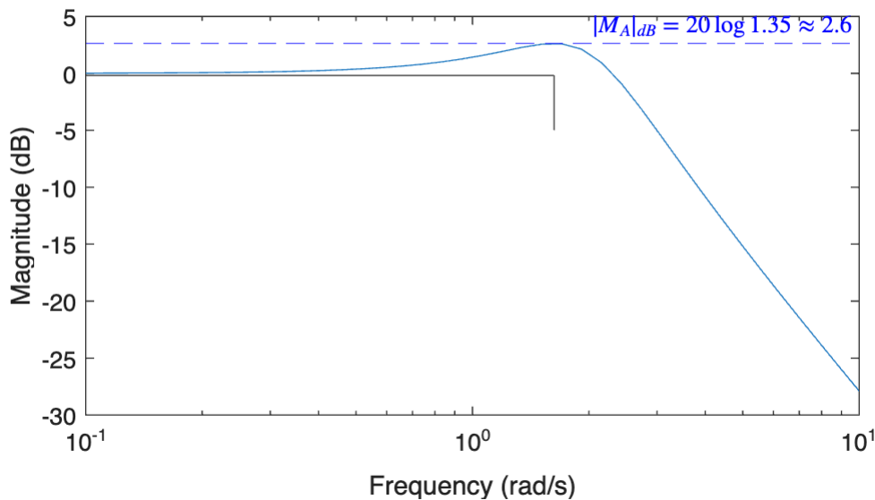
Bode Diagram
