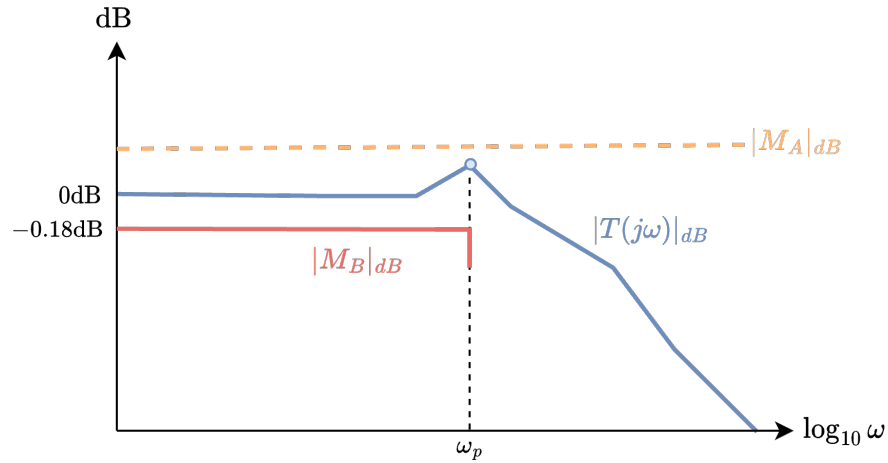
Figure 11.6: Simplified stay-above and stay-below bounds for the magnitude response of T(j\omega) .
