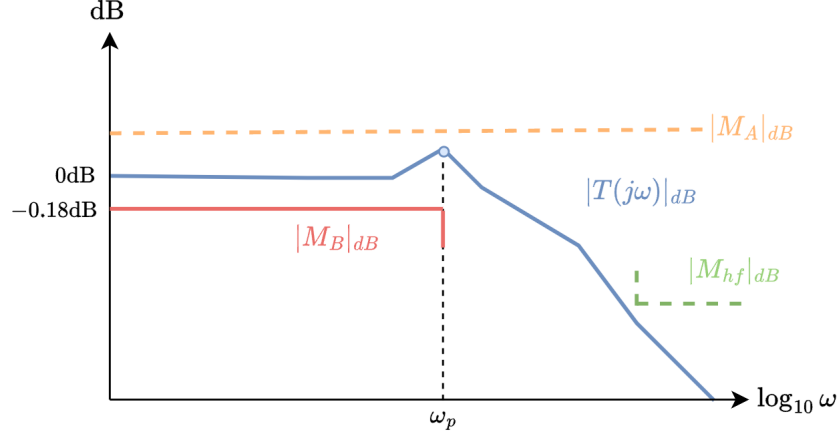
Figure 11.7: Simplified stay-above and stay-below bounds for the magnitude response of T(j\omega) , including high-frequency stay-below bound.
